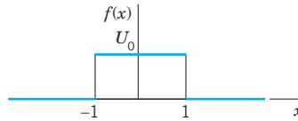
Fig. 298. Initial temperature in Example 1
