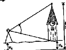
FIG. 24.27. DETERMINATION OF ROH
