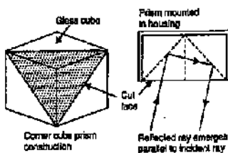
FIG. 24.5. CORNER CUBE PRISM
