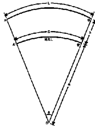
FIG. 3.34. REDUCTION TO MEAN SEA LEVEL
