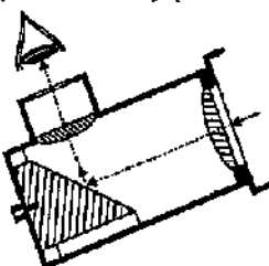
FIG. 9.21. DIAGONAL EYE-PIECE.
