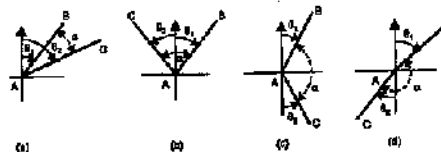
FIG. 5.6. CALCULATION OF ANGLES FROM BEARINGS.
