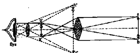
FIG. 9.16 OPTICAL DIAGRAM OF TELESCOPE
