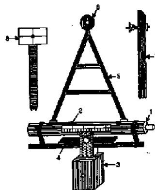
FIG. 14.9. CEYLON GHAT TRACER.
