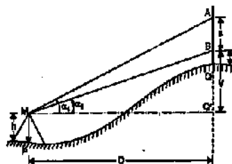
FIG. 22.20. TANGENTIAL METHOD : ANGLES OF ELEVATION
