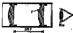
FIG. 9.19. HUYGEN'S EYE-PIECE
