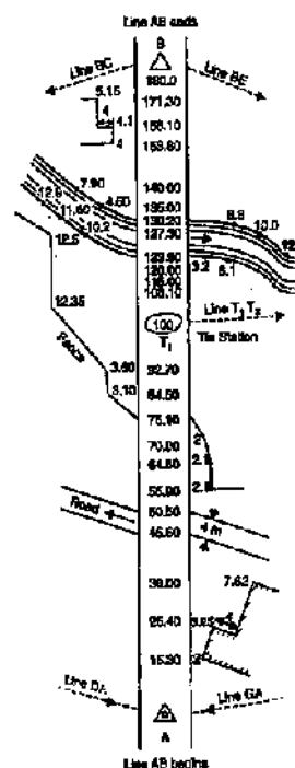
FIG. 4.12. DOUBLE LINE BOOKING.
