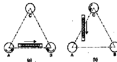
FIG. 6.7. LEVELLING UP WITH THREE FOOT SCREWS
