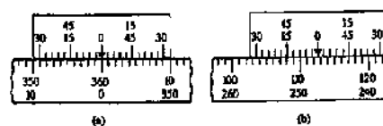
FIG. 1.10 DOUBLE-FOLDED VERNIER.
