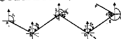
FIG. 5.7. CALCULATION OF BEARINGS FROM ANGLES.
