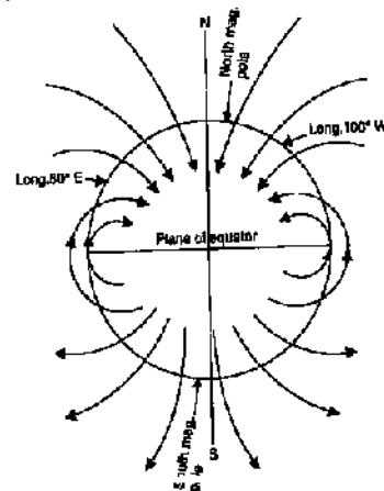
FIG. 5.10. CROSS-SECTION OF EARTH'S MAGNETIC FIELD.
