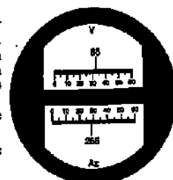
FIG. 22.40. VERTICAL AND HORIZONTAL CIRCLE READINGS IN WILD ROD TACHEOMETER.
