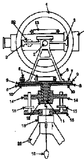
FIG. 6.2. THE ESSENTIALS OF A TRANSIT.
