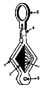
FIG. 14.6. BUREL HAND LEVEL.
