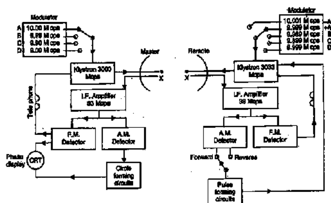
FIG. 24.9 BLOCK DIAGRAM OF THE TELLURIMETER SYSTEM.
