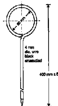
FIG. 3.15. ARROW.
