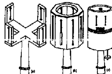
FIG. 4.14. VARIOUS FORMS OF CROSS STAFF.
