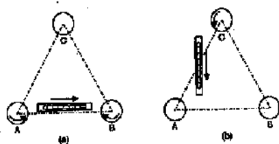
FIG. 9.29. LEVELLING-UP WITH THREE FOOT SCREWS.
