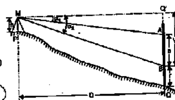
FIG. 22.21. TANGENTIAL METHOD : ANGLES OF DEPRESSION
