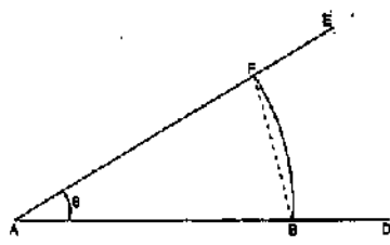
FIG. 1.16 MEASUREMENT OF AN ANGLE WITH THE SCALE OF CHORDS.
