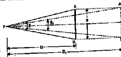
FIG. 22.13. PRINCIPLE OF SUBTENSE METHOD.
