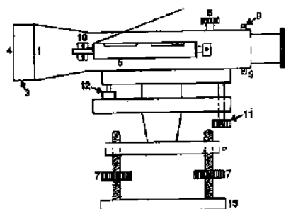
FIG. 9.9 TILTING LEVEL.
