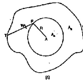
FIG. 12.12. THEORY OF PLANIMETER.
