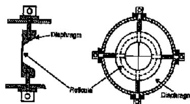
FIG. 9.22. DIAPHRAGM AND RETICULE.
