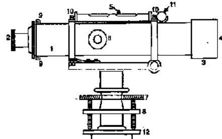
FIG. 9.2. DUMPY LEVEL
