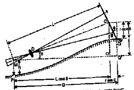
FIG. 22.7. ELEVATED SIGHT : NORMAL HOLDING.
