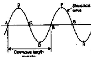
FIG. 24.1 PERIODIC SINUSOIDAL WAVES.
