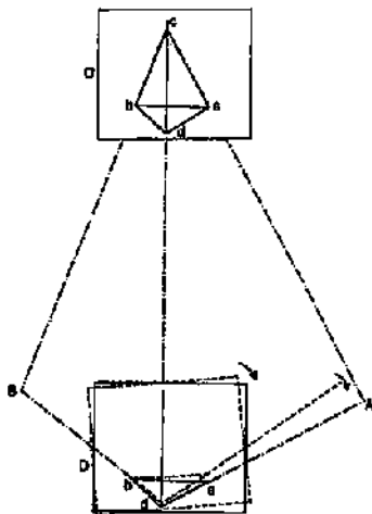
FIG. 11.26. TWO-POINT PROBLEM.
