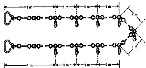
FIG. 3.3 10-METRE CHAIN
