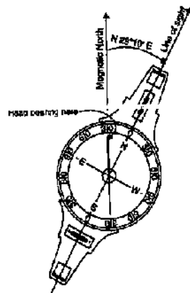
FIG. 5.15. SURVEYOR'S COMPASS (PLAN).
