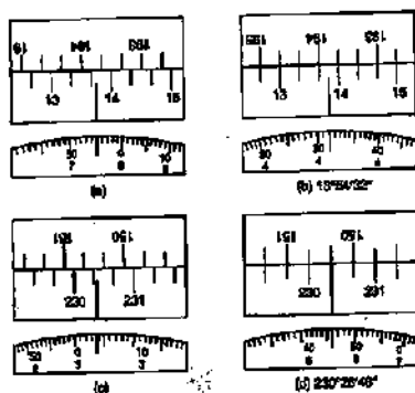
FIG. 19.7. VIEWS IN MICROMETER OF WILD T-2 THEODOLITE.
