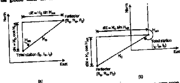
FIG. 24.33. COMPUTATION OF EAST AND NORTH COORDINATES OF THE REFLECTOR
