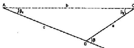
FIG. 3.33. CORRECTION FOR HORIZONTAL ALIGNMENT
