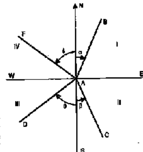
FIG. 5.2 Q.B. SYSTEM.
