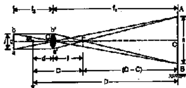
FIG. 22.4. PRINCIPLE OF STADIA METHOD.
