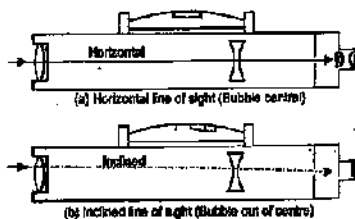
FIG. 21.3. CONVENTIONAL LEVEL.
