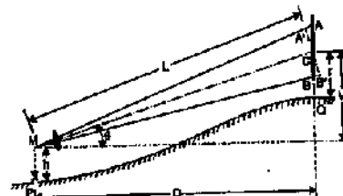
FIG. 22.11. ANALLACTIC LENS : INCLINED SIGHT.
