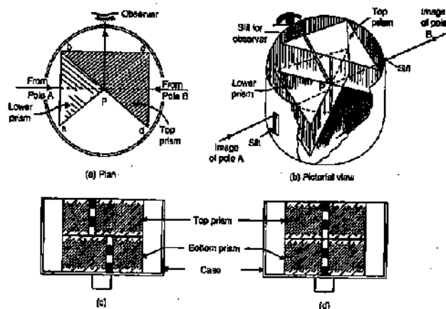
FIG. 3.21. OPTICAL LINE RANGER
