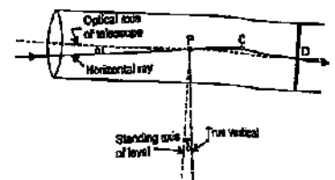
FIG. 21.4. PRINCIPLE OF COMPENSATOR.
