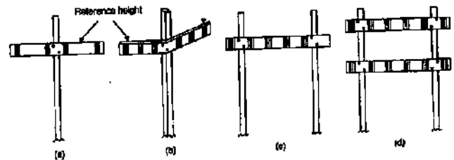
FIG. 20.7. VARIOUS FORMS OF SIGHT RAILS.
