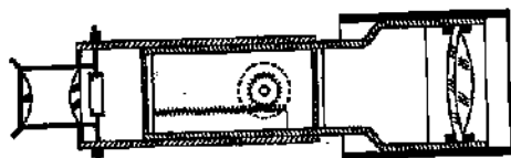
FIG. 9.24. EXTERNAL FOCUSING TELESCOPE.
