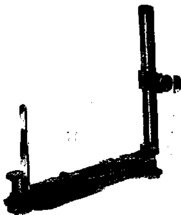
FIG. 14.5. INDIAN PATTERN CLINOMETER.
