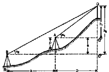
FIG. 15.8. INSTRUMENT AXES AT VERY DIFFERENT LEVELS.
