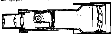
FIG. 9.25. INTERNAL FOCUSING TELESCOPE.
