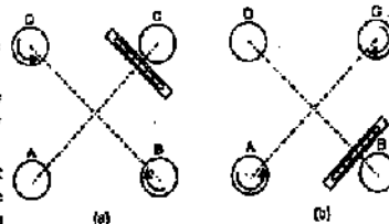
FIG. 9.30. LEVELLING-UP WITH FOUR-FOOT
