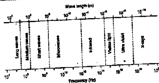
FIG. 24.2 ELECTROMAGNETIC SPECTRUM.
