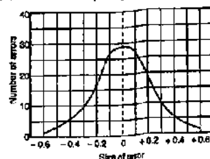
FIG. 2.1 PROBABILITY CURVE.
