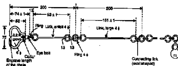
FIG. 3.6. DETAILS OF A METRIC CHAIN
