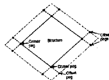
FIG. 20.11. OFFSET PEGS.
