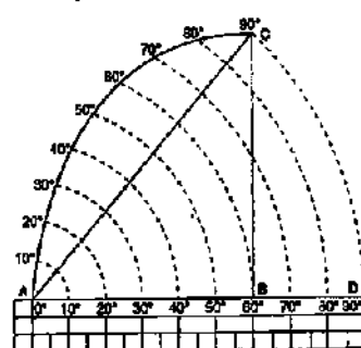
FIG. 1.14. CONSTRUCTION OF A CHORD SCALE.
