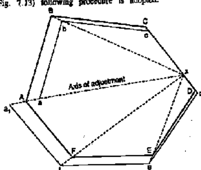
FIG. 7.13. AXIS METHOD OF BALANCING TRAVERSE.
