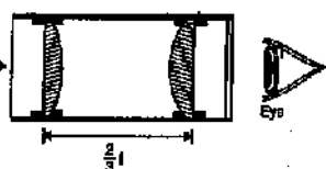
FIG. 9.18. RAMSDEN EYE-PIECE
