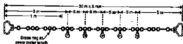
FIG. 1.5. 30-METRE CHAIN
