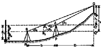
FIG. 15.7. INSTRUMENT AXES AT DIFFERENT LEVELS.
