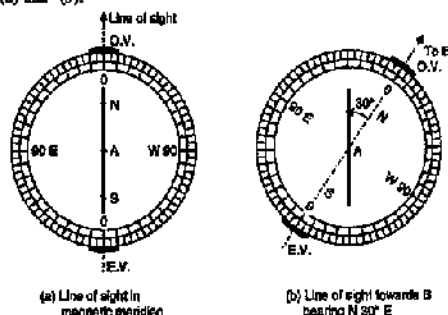
FIG. 5.16. SYSTEM OF GRADUATIONS IN THE SURVEYOR'S COMPASS.
