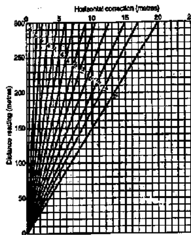
FIG. 22.24. REDUCTION DIAGRAM FOR HORIZONTAL CORRECTION.
