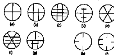
FIG. 9.23. CROSS-HAIRS
