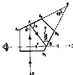
FIG. 4.17. PRISM SQUARE.
