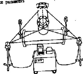
FIG. 23.11. RMS (REMOTE MEASURING SYSTEM) INTERSECTION METHOD
