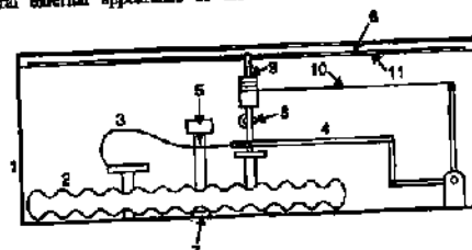
FIG. 9.54. DIAGRAMMATIC SECTION OF AN ANEROID
