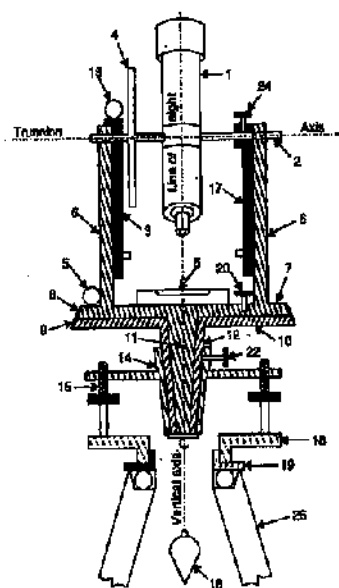
FIG. 6.1. THE ESSENTIALS OF A TRANSIT.
