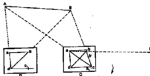
FIG. 11.25. TWO-POINT PROBLEM.
