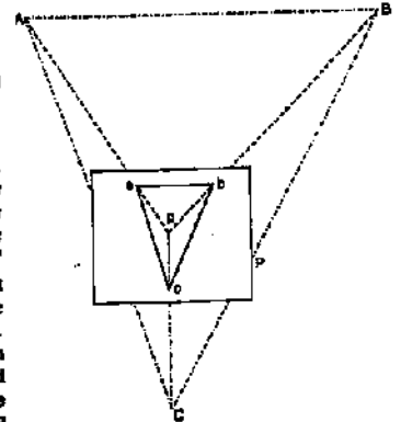
FIG. 11.13. CONDITION OF CORRECT ORIENTATION
