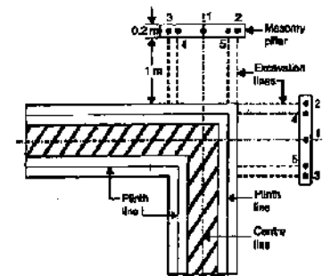
FIG. 20.13. SETTING OUT USING MASONRY PILLARS.
