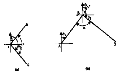
FIG. 5.5. CALCULATION OF ANGLES FROM BEARINGS.
