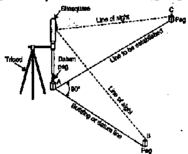
FIG. 21.2. SETTING OUT A RIGHT ANGLE.
