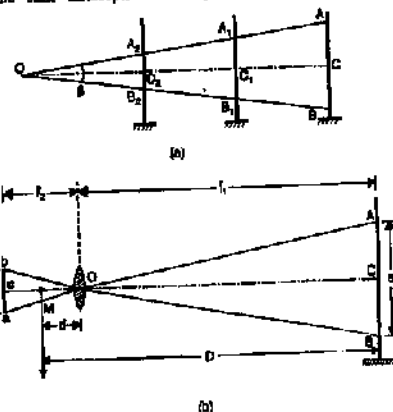
FIG. 22.3. PRINCIPLE OF STADIA METHOD.
