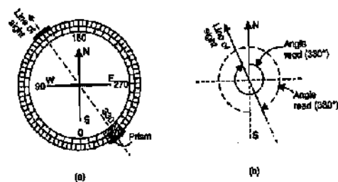
FIG. 5.13. SYSTEM OF GRADUATION IN PRISMATIC COMPASS.
