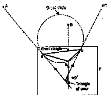
FIG. 11.17. TRIANGLE OF ERROR METHOD
