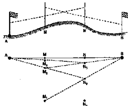
FIG. 3.22. RECIPROCAL RANGING.
