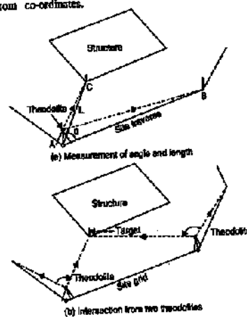
FIG. 20.10. POSITIONING OF DESIGN POINTS.
