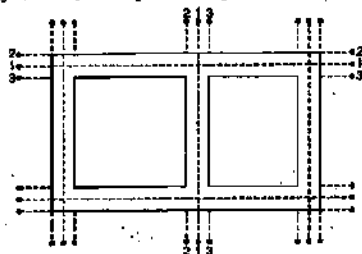
FIG. 20.12. SETTING OUT WITH THE HELP OF PEGS.
