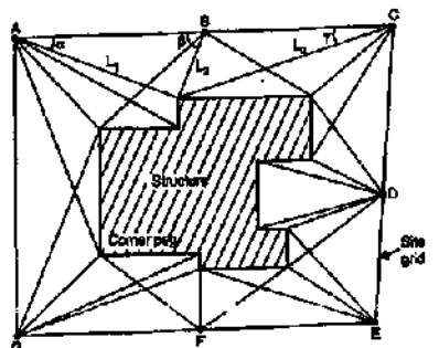
FIG. 20.3 SITE GRID.
