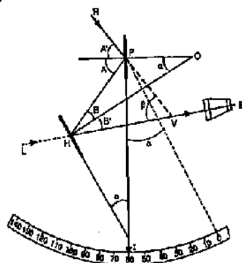
FIG. 14.15. OPTICAL DIAGRAM OF A SEXTANT.
