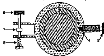
FIG. 6.4. CLAMP AND TANGENT SCREW FOR LOWER PLATE.
