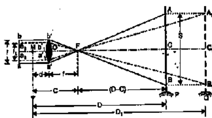
FIG. 22.14. VERTICAL BASE SUBTENSE METHOD.
