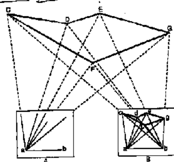
FIG. 11.9. INTERSECTION.
