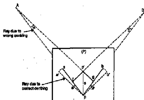
FIG. 11.27. ERROR DUE TO WRONG CENTRING.
