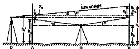
FIG. 16.4 TWO-PEG TEST (METHOD B).
