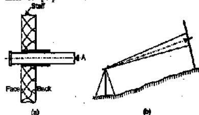
FIG. 22.19. THE PEEP SIGHT.
