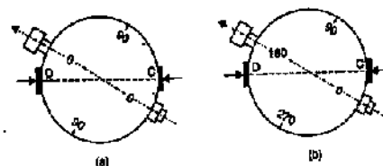
FIG. 4.11. EXAMPLES OF VERTICAL CIRCLE GRADUATION.
