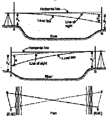
FIG. 9.41. RECIPROCAL LEVELLING.
