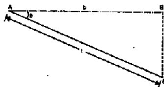
FIG. 3.29. CORRECTION FOR SLOPE.
