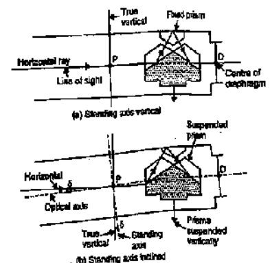
FIG. 21.5. THE COMPENSATOR SYSTEM.
