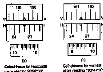
FIG. 19.2 VIEW IN MICROPTIC OF WATTS MICROPTIC THEODOLITE NO. 1
