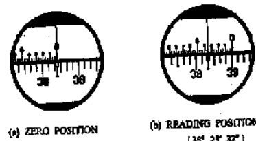
FIG. 19.4. EXAMPLE OF HORIZONTAL CIRCLE READING.
