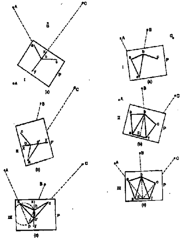
FIG. 11.15. THREE-POINT PROBLEM : BESSEL'S METHOD.
