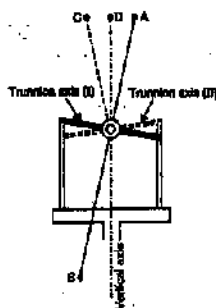
FIG. 18.3. SPIRE TEST.
