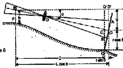
FIG. 22.8. DEPRESSED SIGHT: NORMAL HOLDING.
