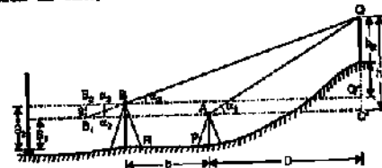
FIG. 15.6. INSTRUMENT AT DIFFERENT LEVELS
