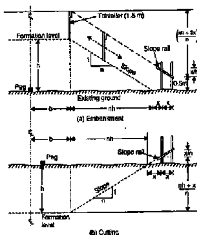
FIG. 20.8. USE OF SLOPE RAILS
