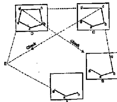
FIG. 11.10 TRAVERSING
