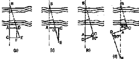
FIG. 4.26. OBSTACLES TO CHAINING.
