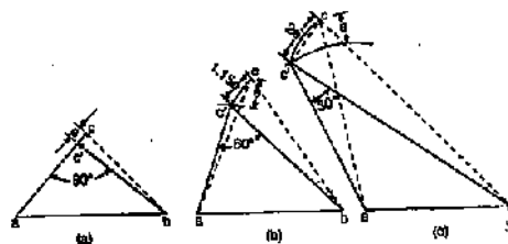
FIG. 4.4. WELL CONDITIONED TRIANGLES.
