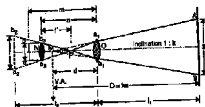
FIG. 22.10. THEORY OF ANALLACTIC LENS.
