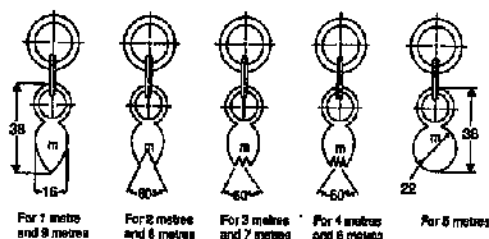
FIG. 3.7. SHAPES OF TALLIES FOR 5 m AND 10 m CHAINS
