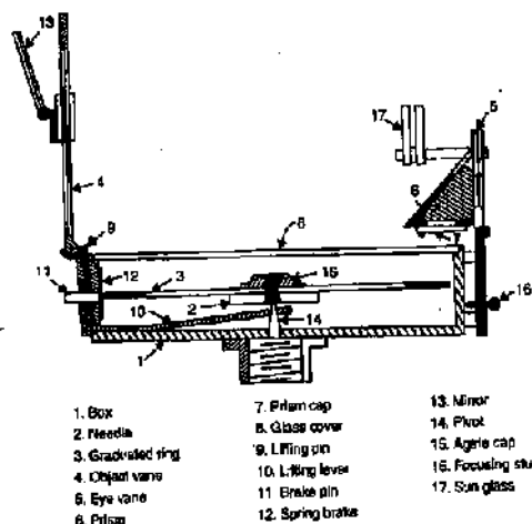
FIG. 5.12. THE PRISMATIC COMPASS.
