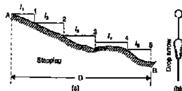
FIG. 3.23. METHOD OF STEPPING.
