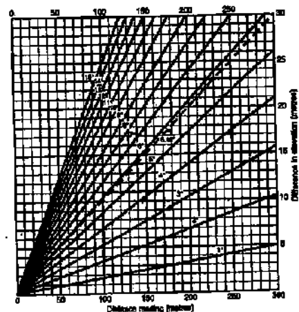
FIG. 22.25. REDUCTION DIAGRAM FOR VERTICAL COMPONENT.
