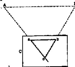
FIG. 11.11. RESECTION AFTER ORIENTATION BY COMPASS.
