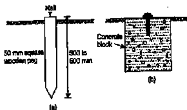
FIG. 20.4. CONTROL POINTS.
