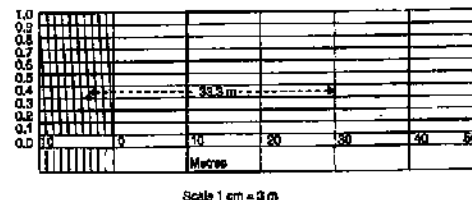
FIG. 1.5 DIAGONAL SCALE.
