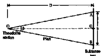
FIG. 22.16. HORIZONTAL BASE SUBTENSE METHOD.
