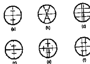
FIG. 22.1. VARIOUS PATTERNS OF STADIA DIAPHRAGM.
