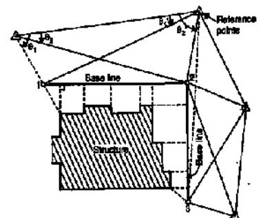
FIG. 20.2 BASE LINE TIED TO REFERENCE POINTS.
