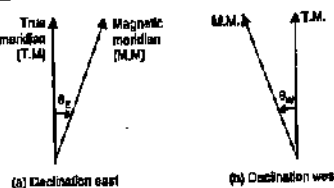
FIG. 5.19. MAGNETIC DECLINATION.
