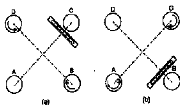
FIG. 6.8. LEVELLING UP WITH FOUR FOOT SCREWS.
