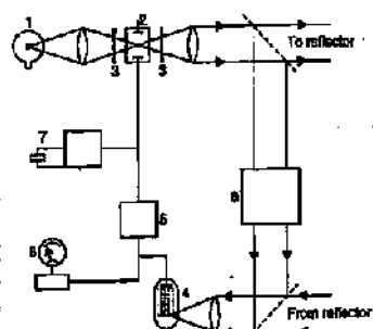
FIG. 24.6. SCHEMATIC DIAGRAM OF THE GEODIMETER.
