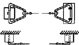
FIG. 3.9 FIELD TESTING OF CHAIN.
