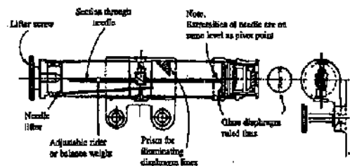
FIG. 6.5. TUBULAR COMPASS. (BY COURTESY OF MESSRS VICKERS INSTRUMENTS LTD.)
