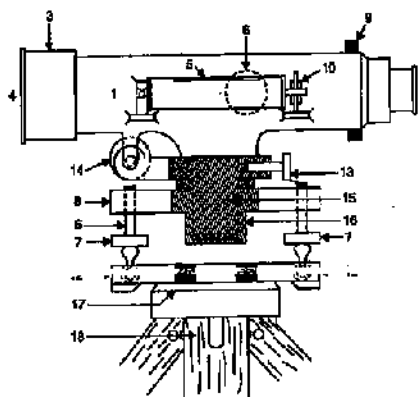
FIG. 9.3 SECTIONAL VIEW OF A DUMPY LEVEL.
