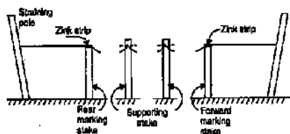
FIG. 3.37. WHEELER'S BASE LINE APPARATUS.
