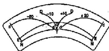
FIG. 22.29. SPECIAL AUTO-REDUCTION DEVICE (HAMMER-FENNEL)
