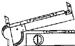
FIG. 14.8. FOOT-RULE CLINOMETER.
