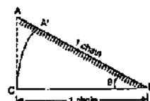
FIG. 3.27. HYPOTENUSAL ALLOWANCE.
