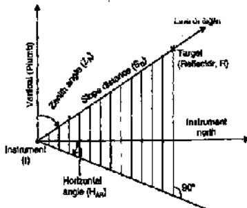
FIG. 24.31. FUNDAMENTAL MEASUREMENTS MADE BY A TOTAL STATION
