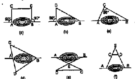
FIG. 4.25. OBSTACLES TO CHAINING.
