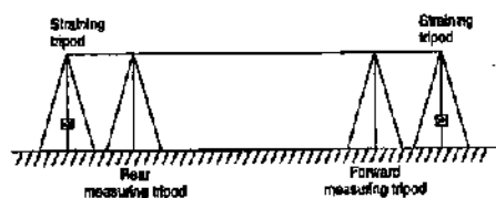
FIG. 3.38. JADERIN'S METHOD.
