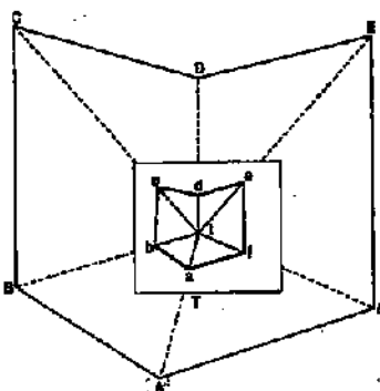
FIG. 11.8. RADIATION.
