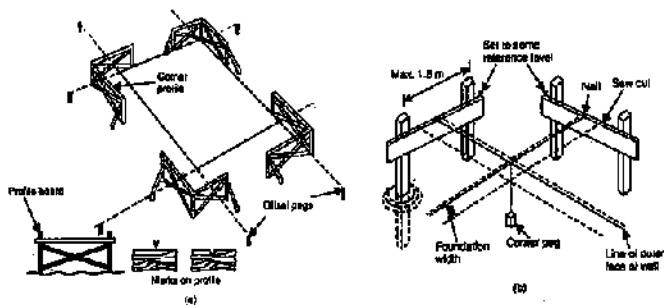
FIG. 20.9. USE OF PROFILE BOARDS.
