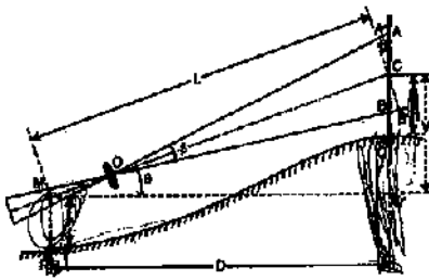
FIG. 22.5. ELEVATED SIGHT : VERTICAL HOLDING.
