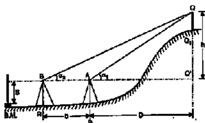
FIG. 15.5. INSTRUMENT AXES AT THE SAME LEVEL
