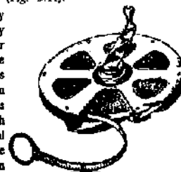
FIG. 3.13. STEEL TAPES ON REEL
