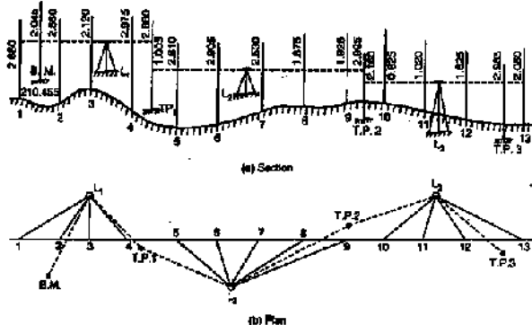
FIG. 9.42. PROFILE LEVELLING.
