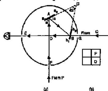
FIG. 4.15. OPTICAL SQUARE.
