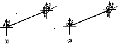
FIG. 5.3. FORE AND BACK BEARINGS.
