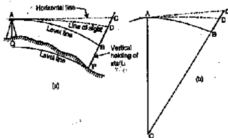
FIG. 9.38. CURVATURE AND REFRACTION.
