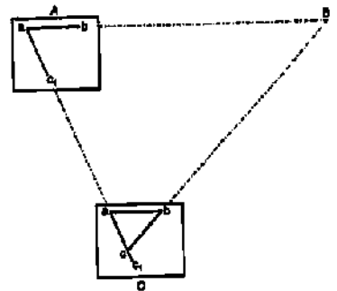
FIG. 11.12. RESECTION AFTER ORIENTATION BY BACKSIGHTING.
