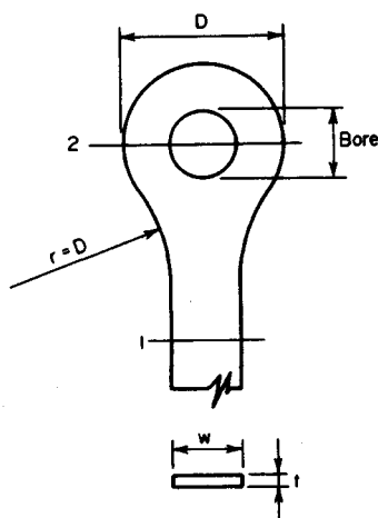
FIGURE 1. Eyebar hanger.
