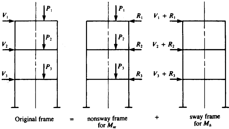
FIGURE 43. Frame models for M_{nt} and M_{lt} .
