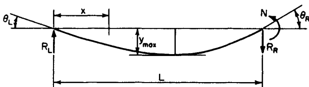
FIGURE 36. Deflection of simple beam under end moment.
